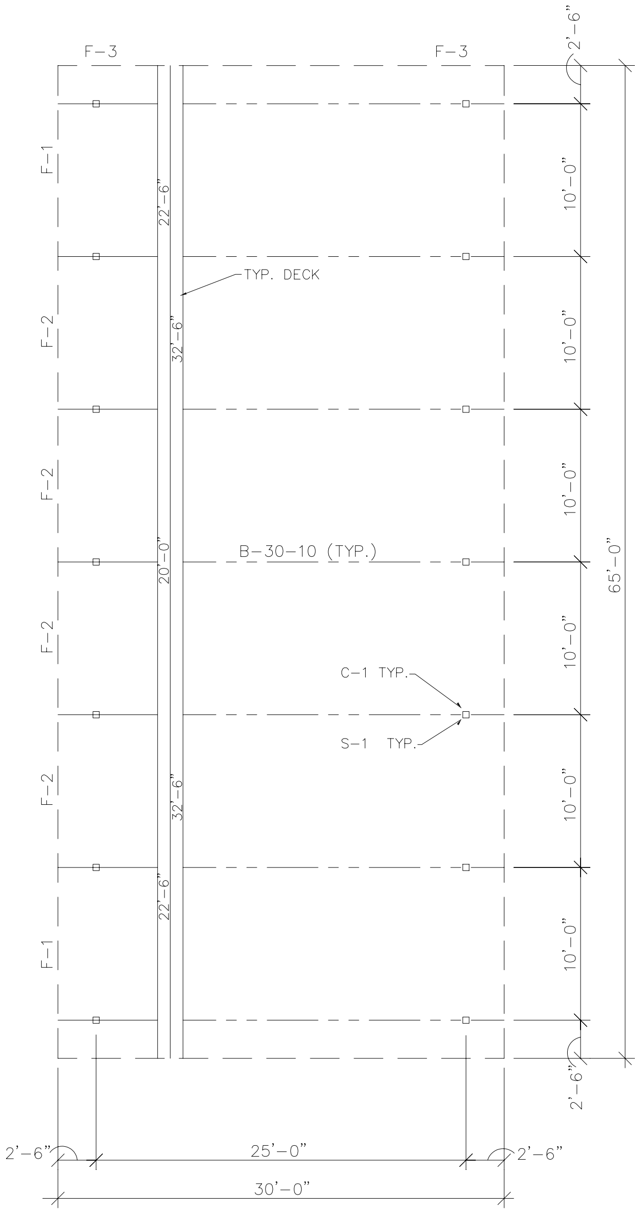
FRAMING PLAN NO SCALE
