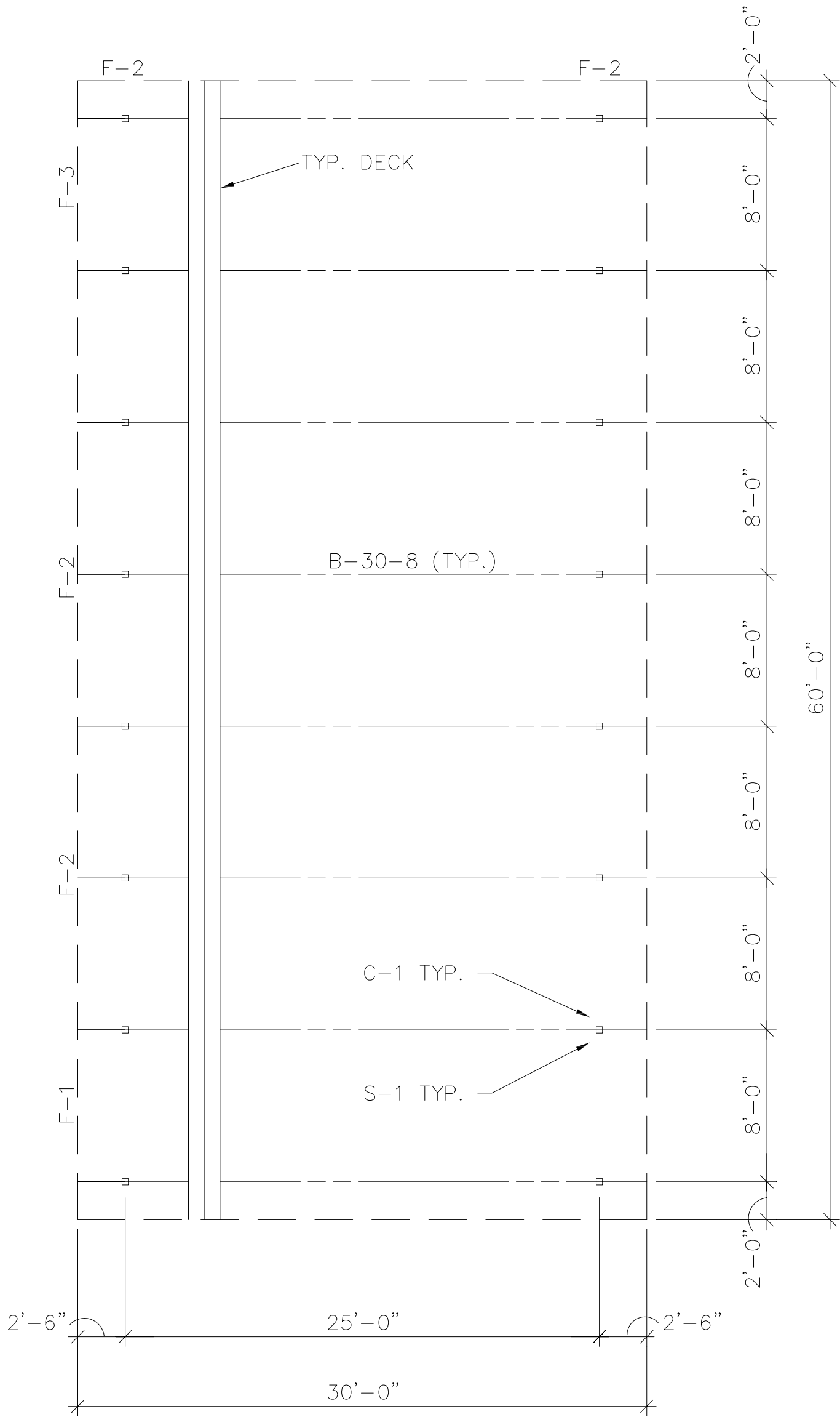
FRAMING PLAN NO SCALE
