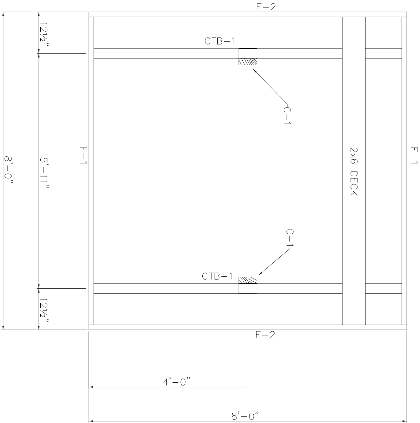
FRAMING PLAN
