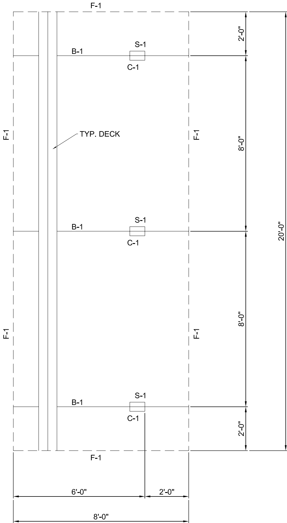
FRAMING PLAN
