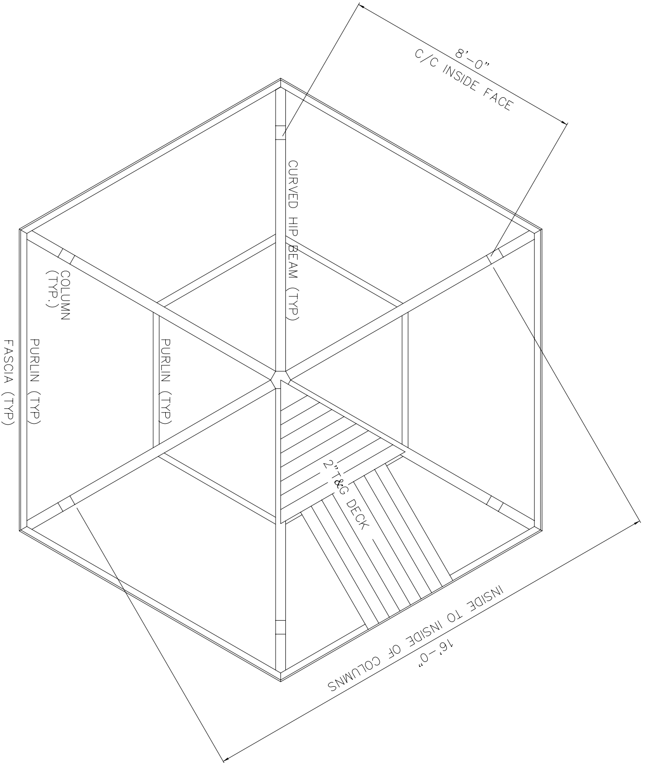
ROOF FRAMING PLAN NO SCALE
