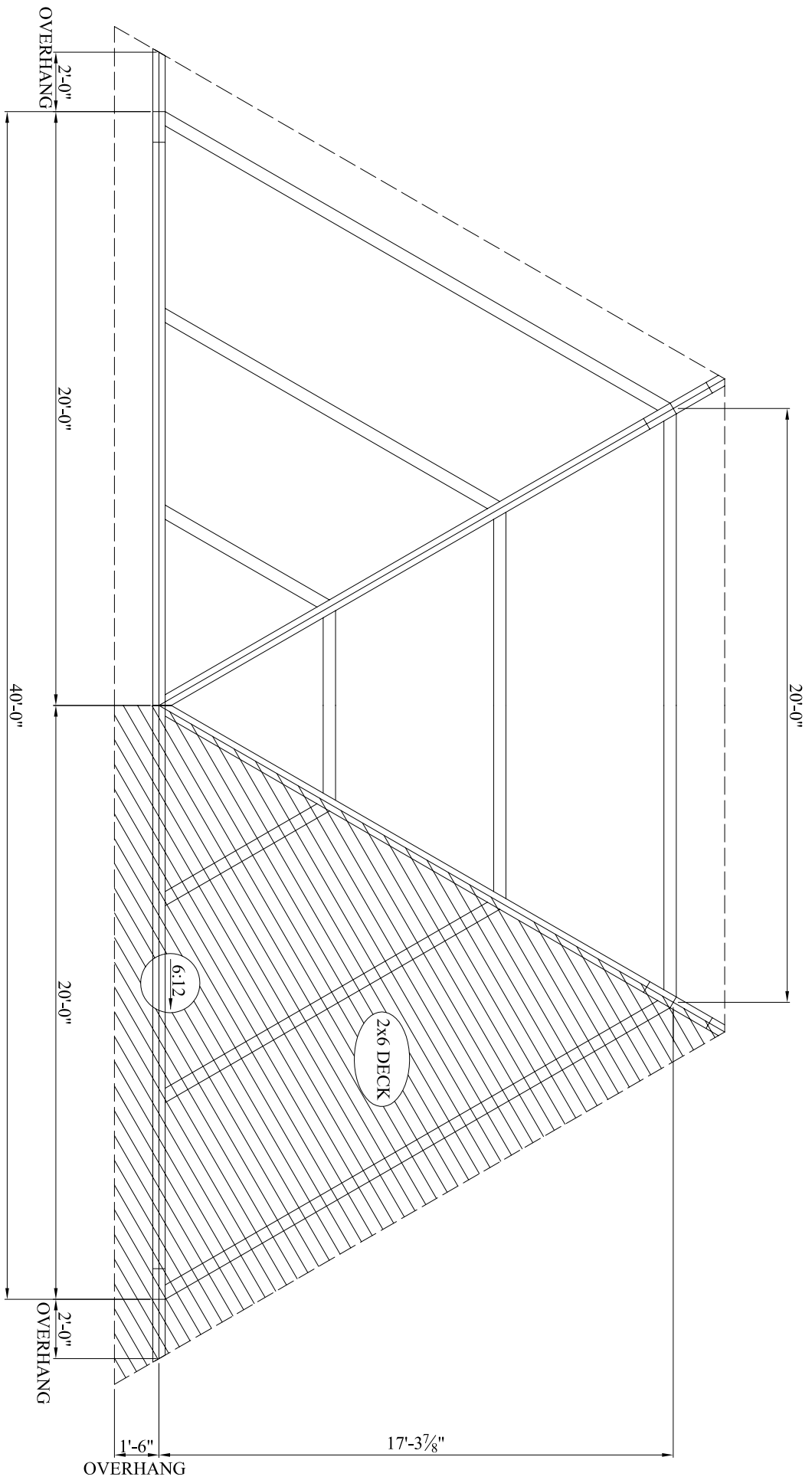
Framing Plan
